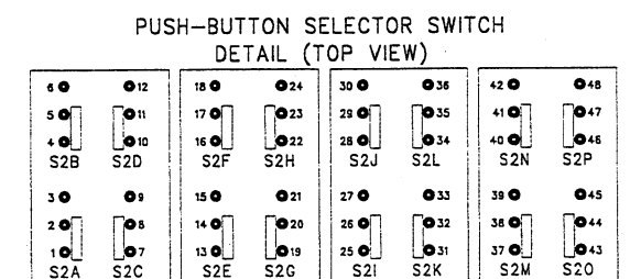
PUSH-BUTTON SELECTOR SWITCH DETAIL (TOP VIEW)
